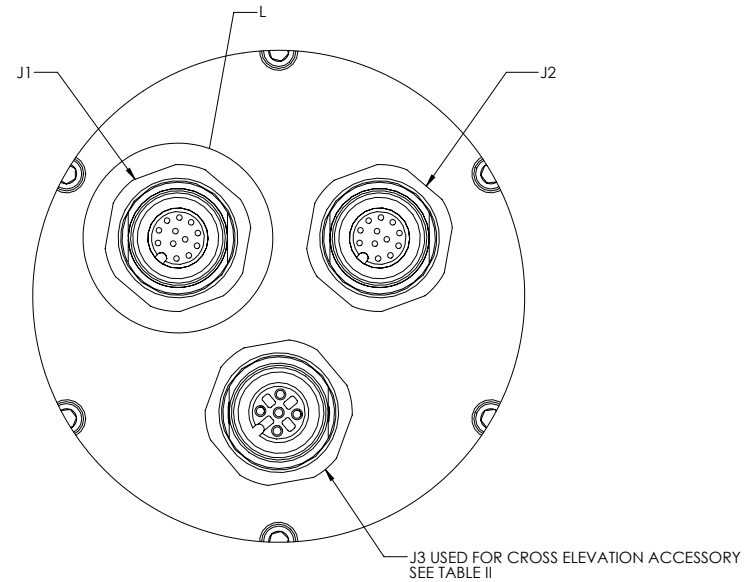
J1 & J2 CONNECTORS SHOWN FROM MATING SIDE MATES WITH TURCK P/N BS 81121-0/PG9 OR RS 12T-*
