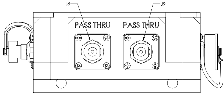
J8 & J9 CONNECTORS SHOWN FROM MATING SIDE MATES WITH N-TYPE MALE CONNECTOR
