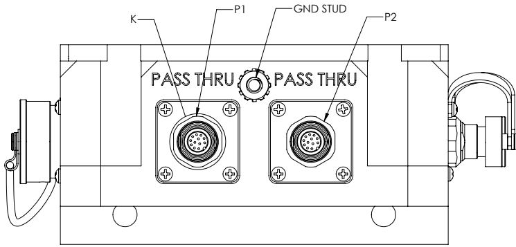
P1 & P2 CONNECTORS SHOWN FROM MATING SIDE MATES WITH TURCK P/N B 81121-0/PG9 OR RK 12T-*
