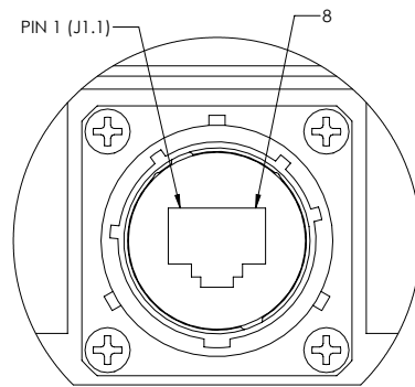
J1 CONNECTOR SHOWN FROM MATING SIDE MATES WITH AMPHENOL P/N - RJF6B
