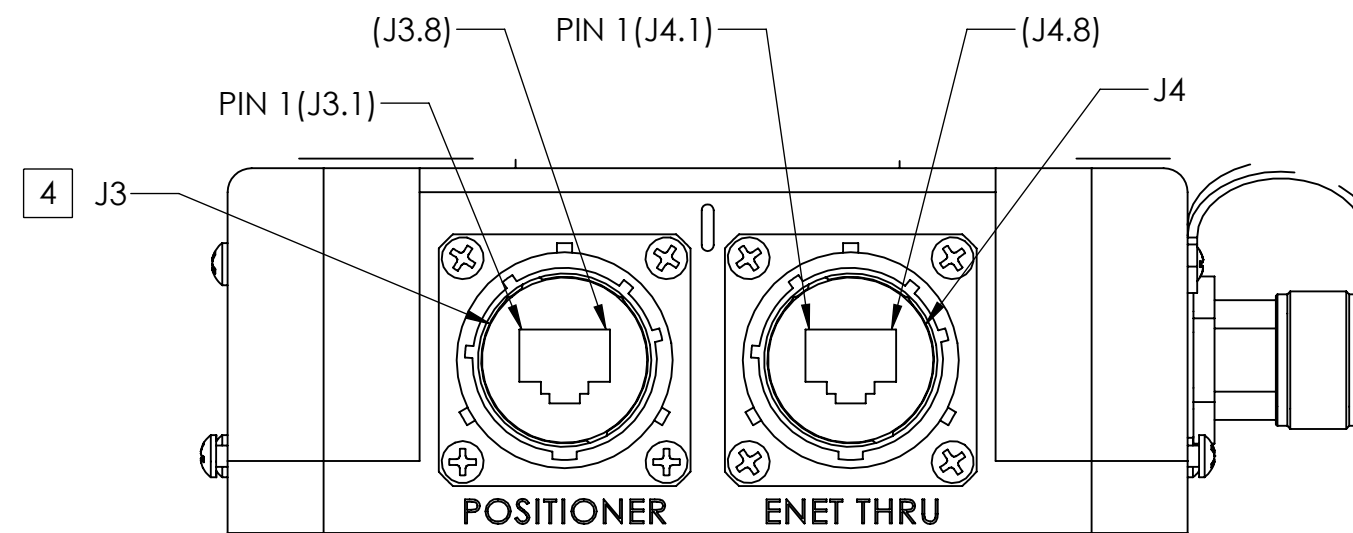
J3 & J4 CONNECTOR SHOWN FROM MATING SIDE MATES WITH AMPHENOL P/N - RJF6B
