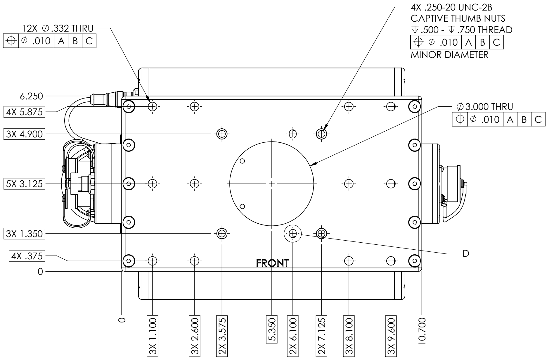
VIEW B-B SCALE 1 : 2 SHEET 2 ZONE D-5
